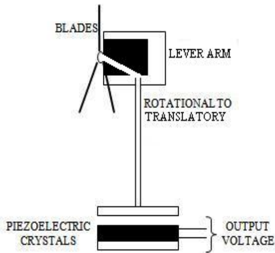
Figure 3: Piezoelectric Wind mill
