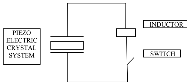
Figure 7: SSHI (Synchronized Switch Harvesting on Inductor) technique
