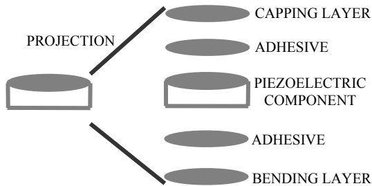
Figure 1: Principle of direct piezoelectric effect
