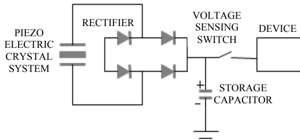
Figure 5: Bridge rectifier type AC to DC converter
