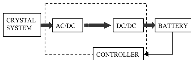
Figure 6: Energy Harvesting Circuit
